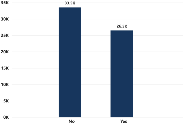
Delivery Status
